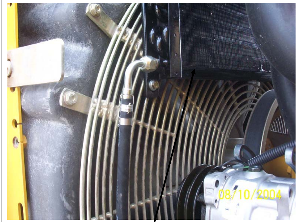
Condenser mounted to rad screen. Keep as low as possible very close to pulley.
