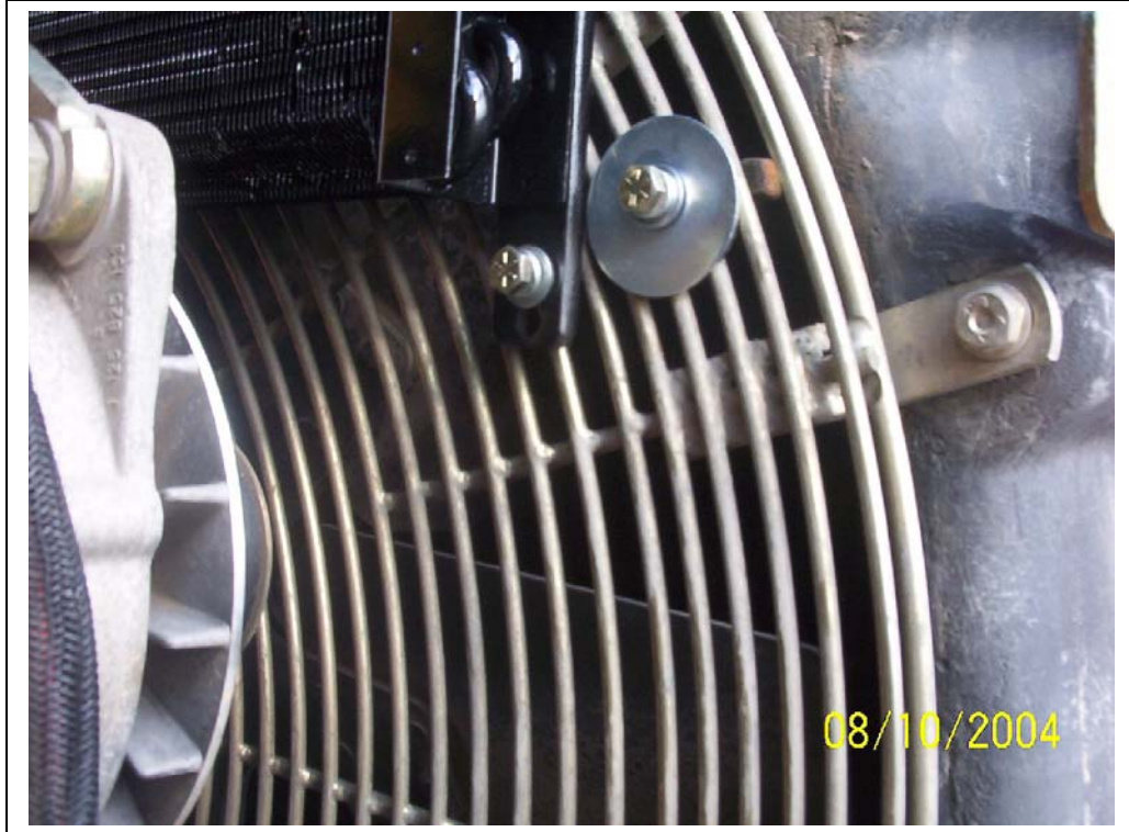
Use this method to fasten the lower side of the condenser. (See drawing)
