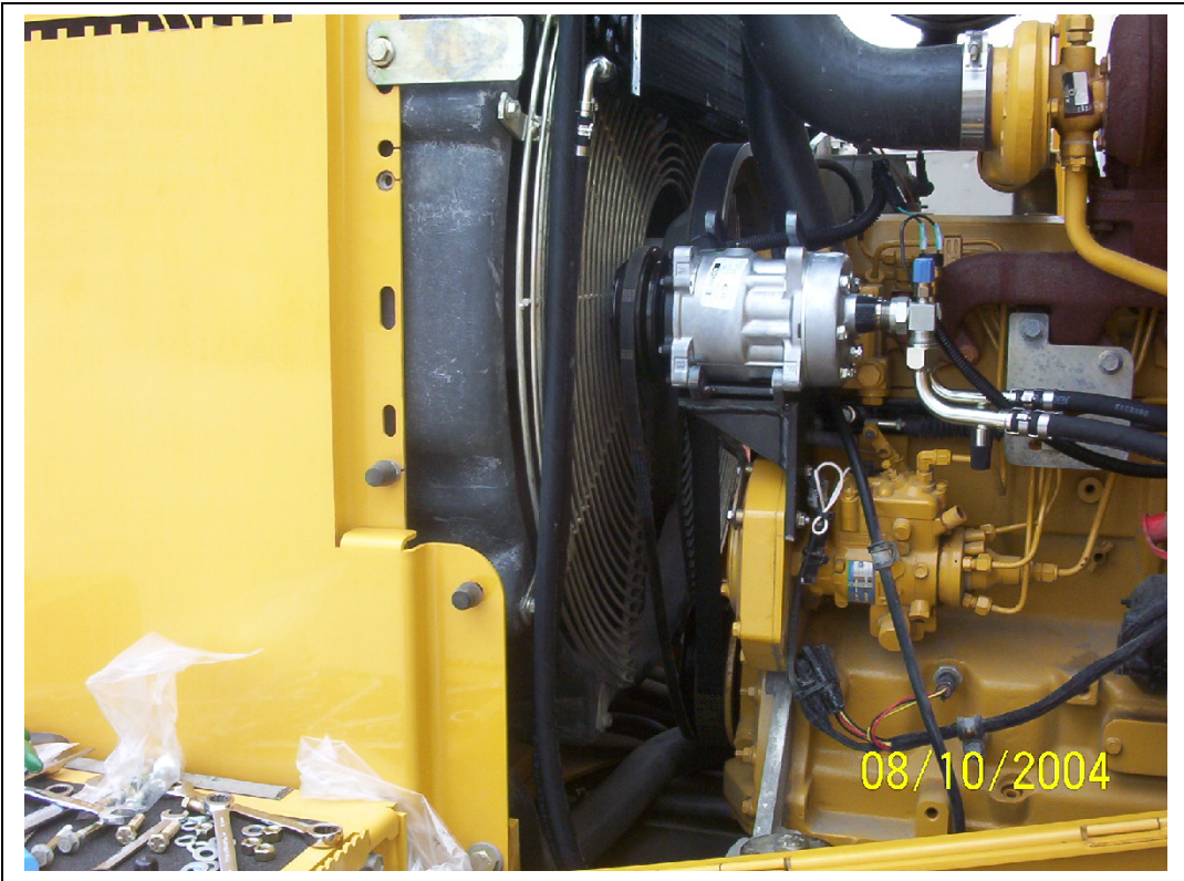
Compressor location
