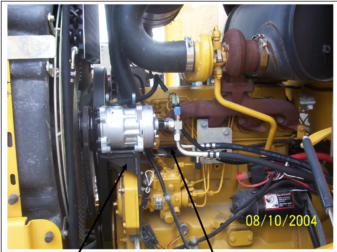
Compressor mount
