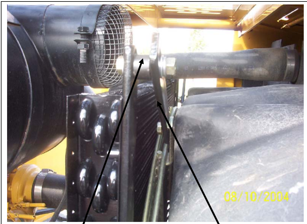
Condenser stiffener bracket. (one on each side) top
